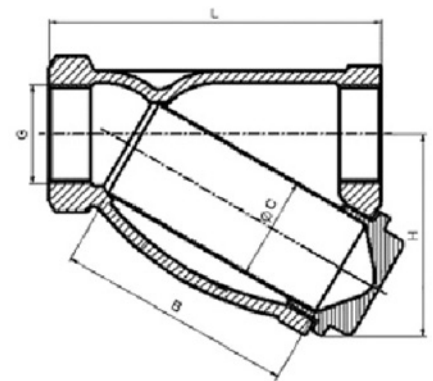
DN10–40
